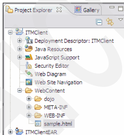
Figure 8-4 Project Explorer
